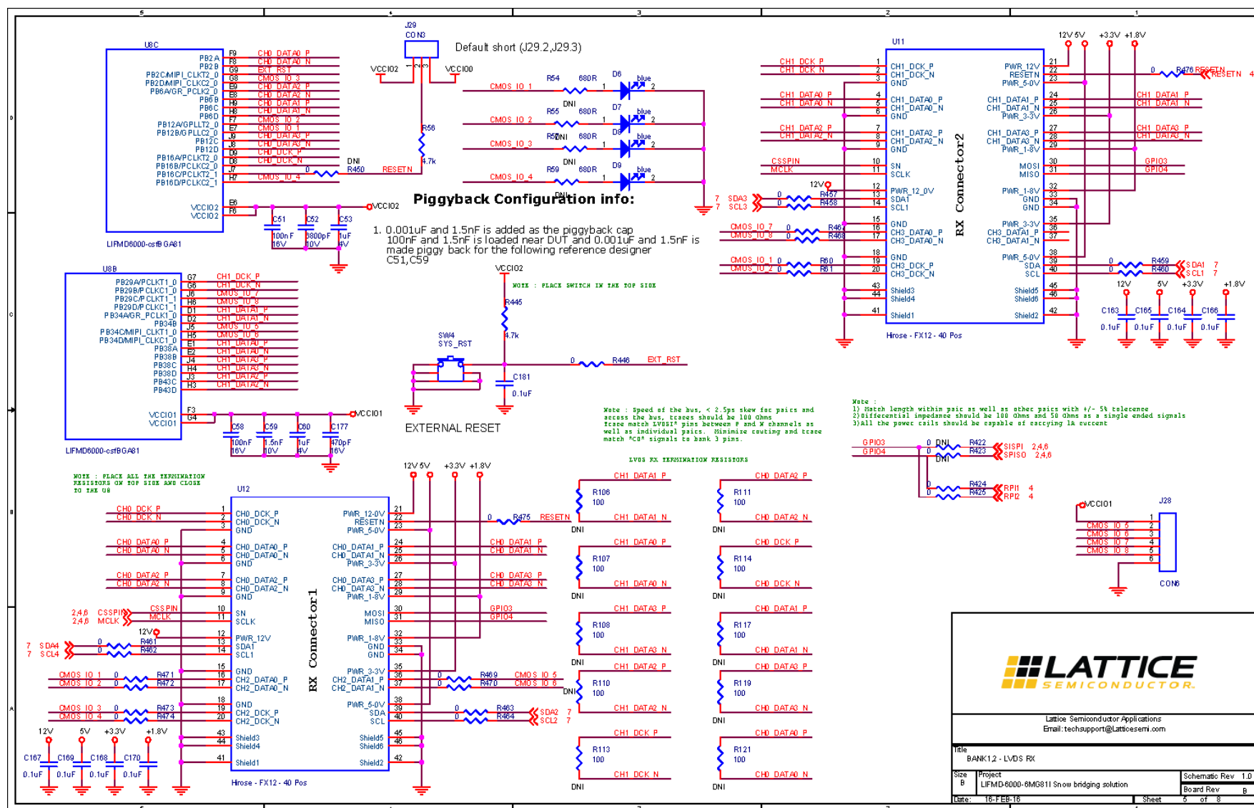
Bank 1, 2 – LVDS Rx
